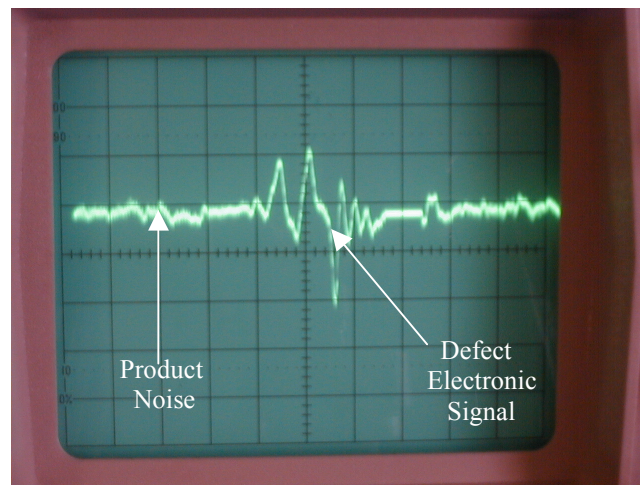
Figure 7 - Signal to Noise Level of Defect Vs Material
