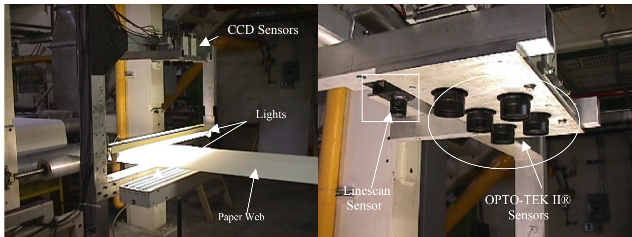
Figure 14 - View of frame support, lighting and sensors
